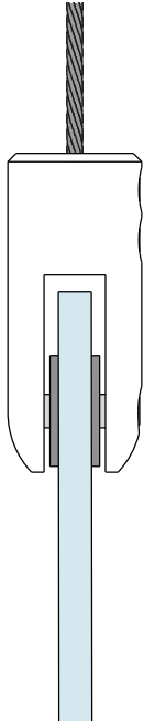
Scale section view, 5/32" glass
