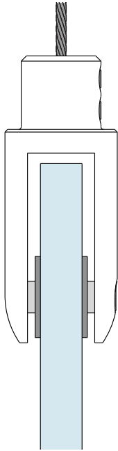
Scale section view, 5/16" glass
