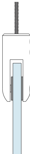
Scale section view, 3/16" glass
