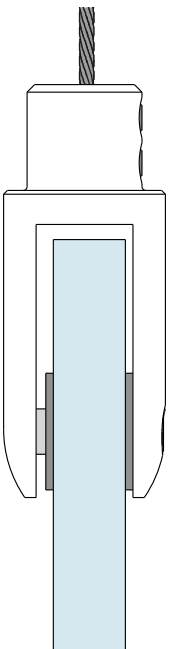
Scale section view, 3/8" glass
